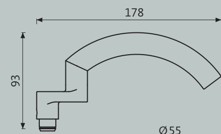
OFFICE H4.0
